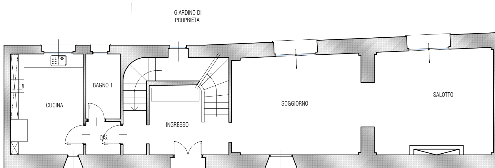
PIANO TERRA
